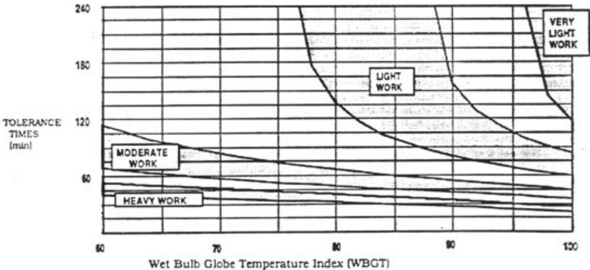
Figure B-2: Estimated Tolerance Times for Four Work Intensities in MOPP4
